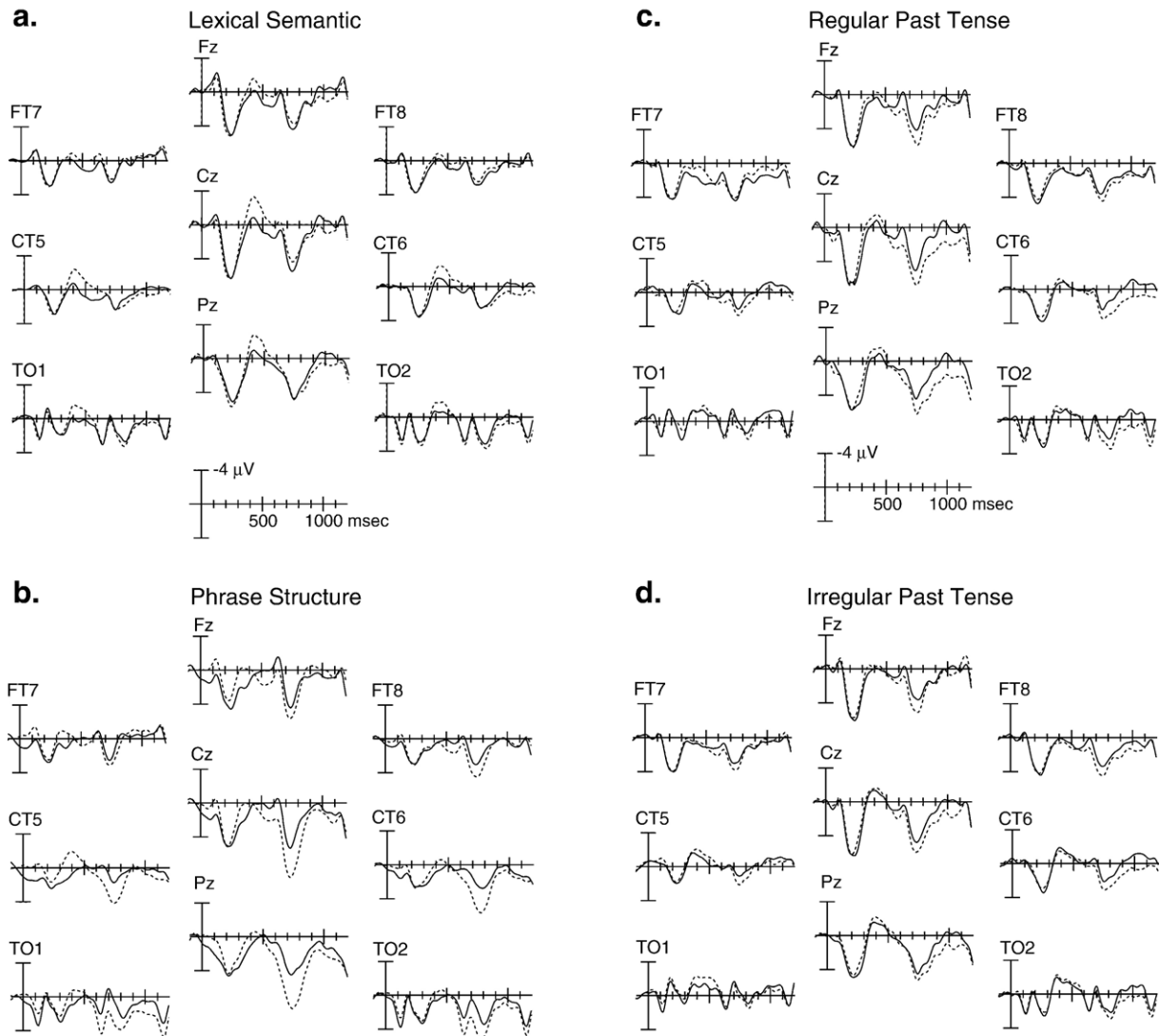
Fig. 1. Grand average ERPs for violation (dashed lines) and control (solid lines) target words in each condition. Waveforms for correct and incorrect target words are superimposed. The ordinate indicates the onset of the target word. Timing is given in milliseconds. Negative voltage is plotted upwards.
